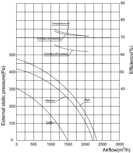
XHBQ-D20PMTG Performance chart
