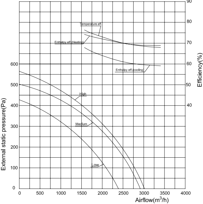
XHBQ-D25PMTG Performance chart
