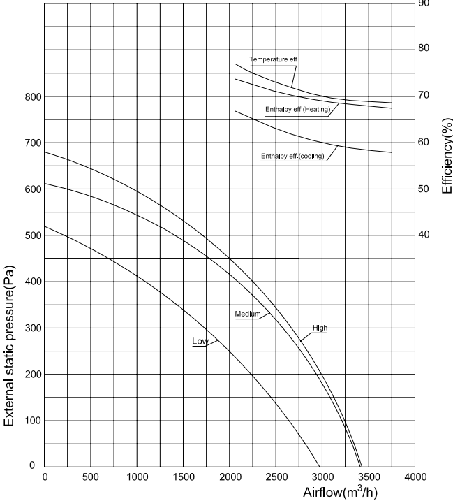
XHBQ-D30PMTG Performance chart
