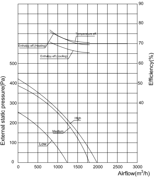
XHBQ-D15PMTG Performance chart
